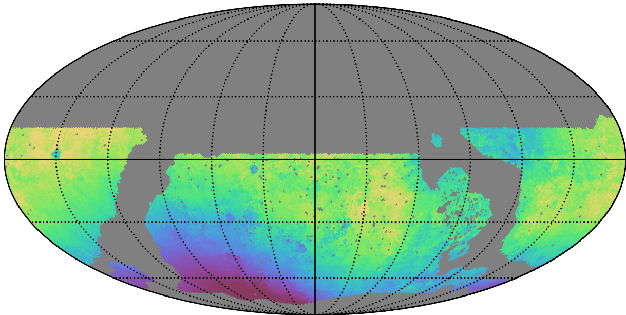
roll_pause_mjdp120_v3.4_10yrs WFD g band: Median solarElong
