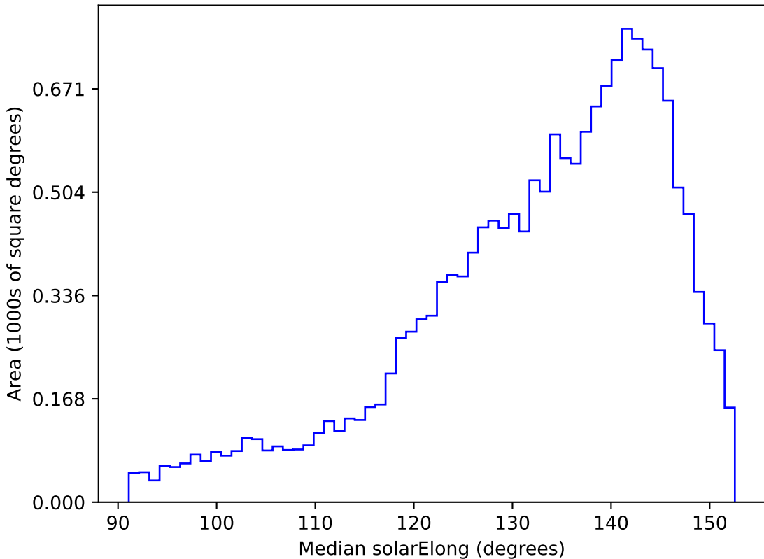
roll_pause_mjdp120_v3.4_10yrs WFD g band: Median solarElong
