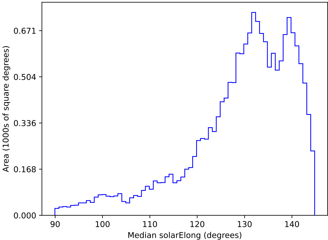
roll_pause_mjdp120_v3.4_10yrs WFD all bands: Median solarElong
