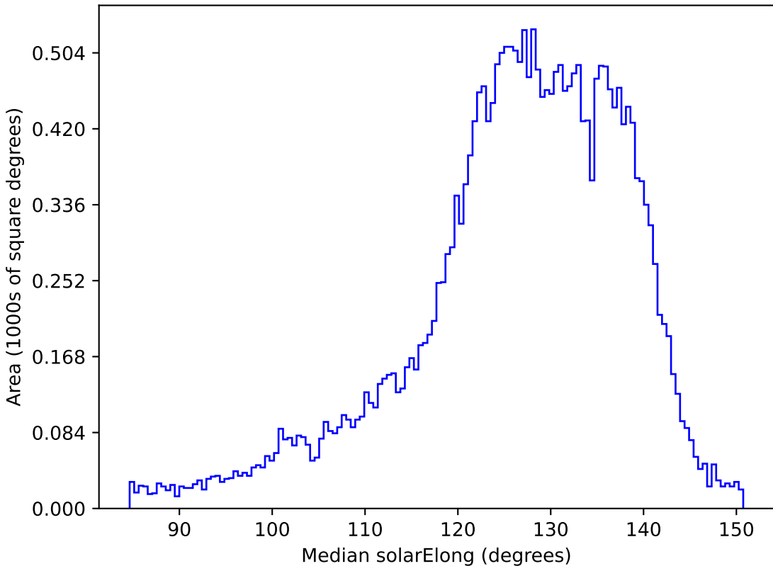
roll_pause_mjdp120_v3.4_10yrs All sky z band: Median solarElong
