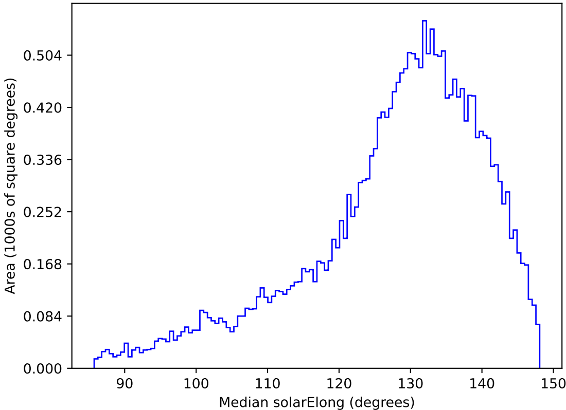
roll_pause_mjdp120_v3.4_10yrs All sky y band: Median solarElong
