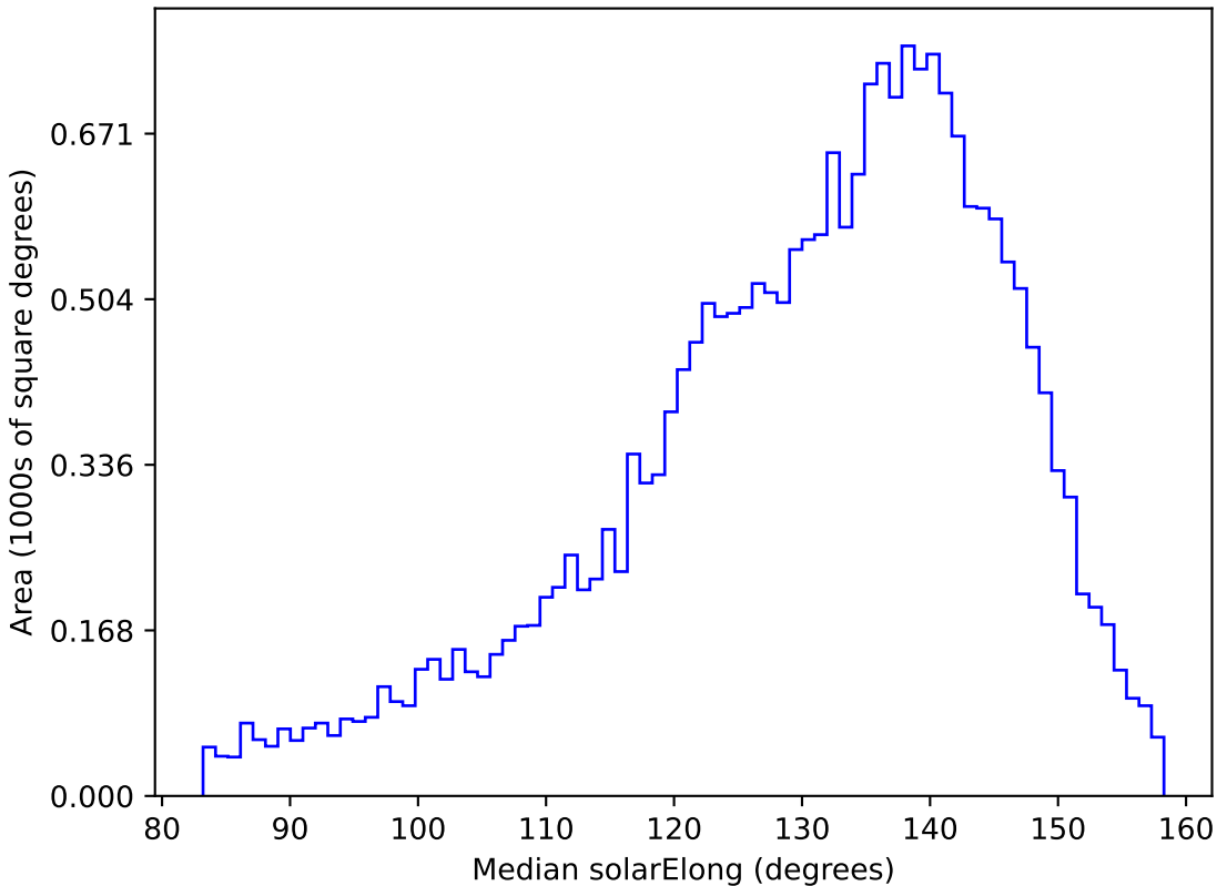
roll_pause_mjdp120_v3.4_10yrs All sky u band: Median solarElong
