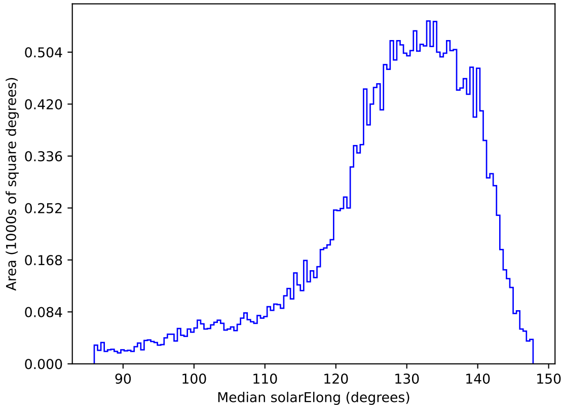
roll_pause_mjdp120_v3.4_10yrs All sky i band: Median solarElong
