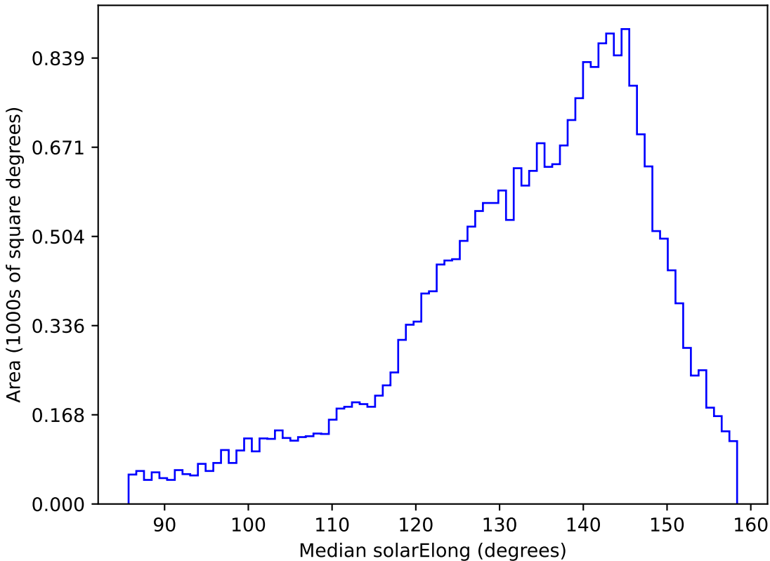
roll_pause_mjdp120_v3.4_10yrs All sky g band: Median solarElong
