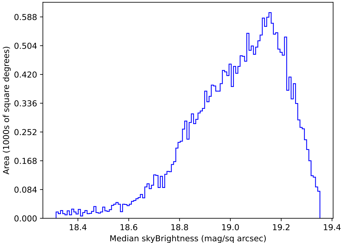
roll_pause_mjdp120_v3.4_10yrs Yr 1 z band: Median skyBrightness
