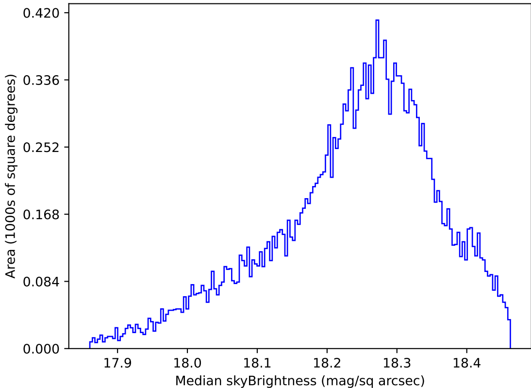
roll_pause_mjdp120_v3.4_10yrs Yr 1 y band: Median skyBrightness
