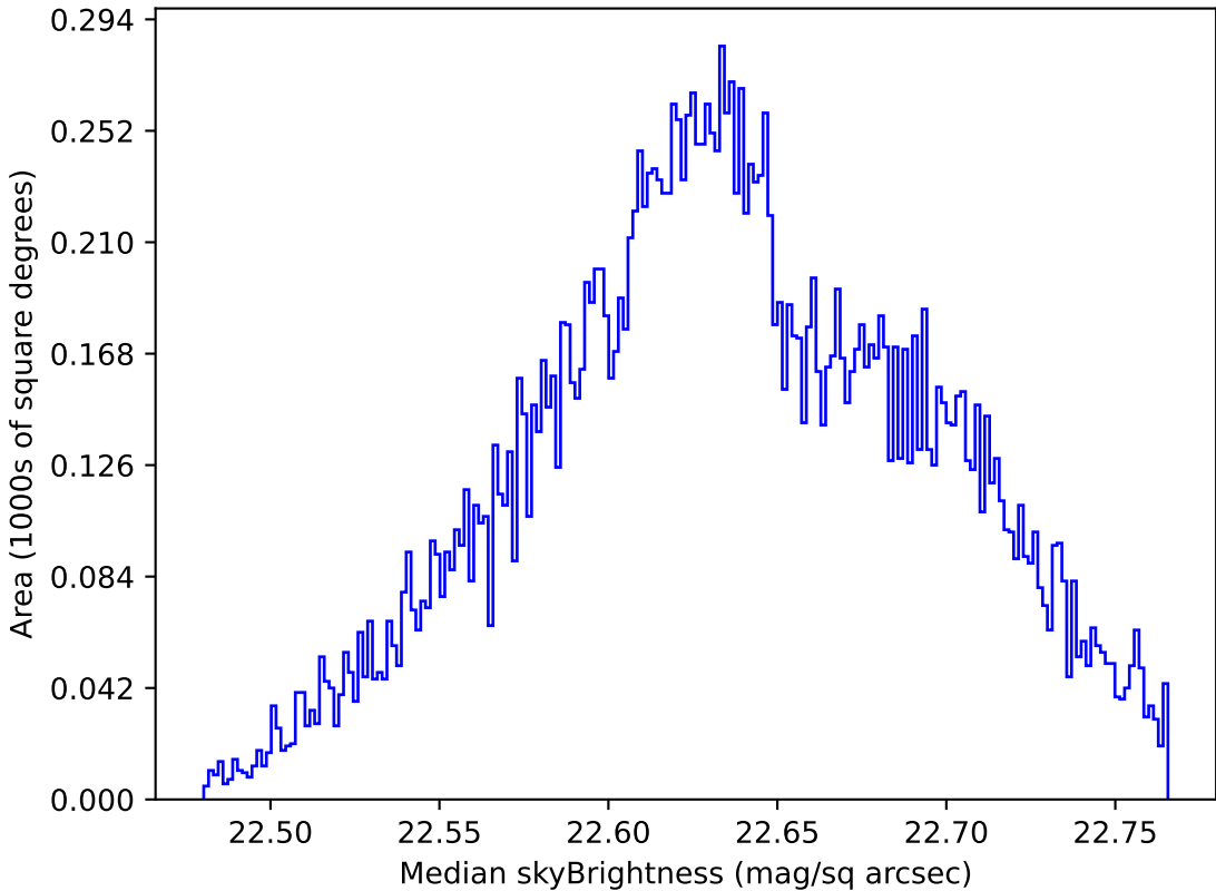
roll_pause_mjdp120_v3.4_10yrs Yr 1 u band: Median skyBrightness
