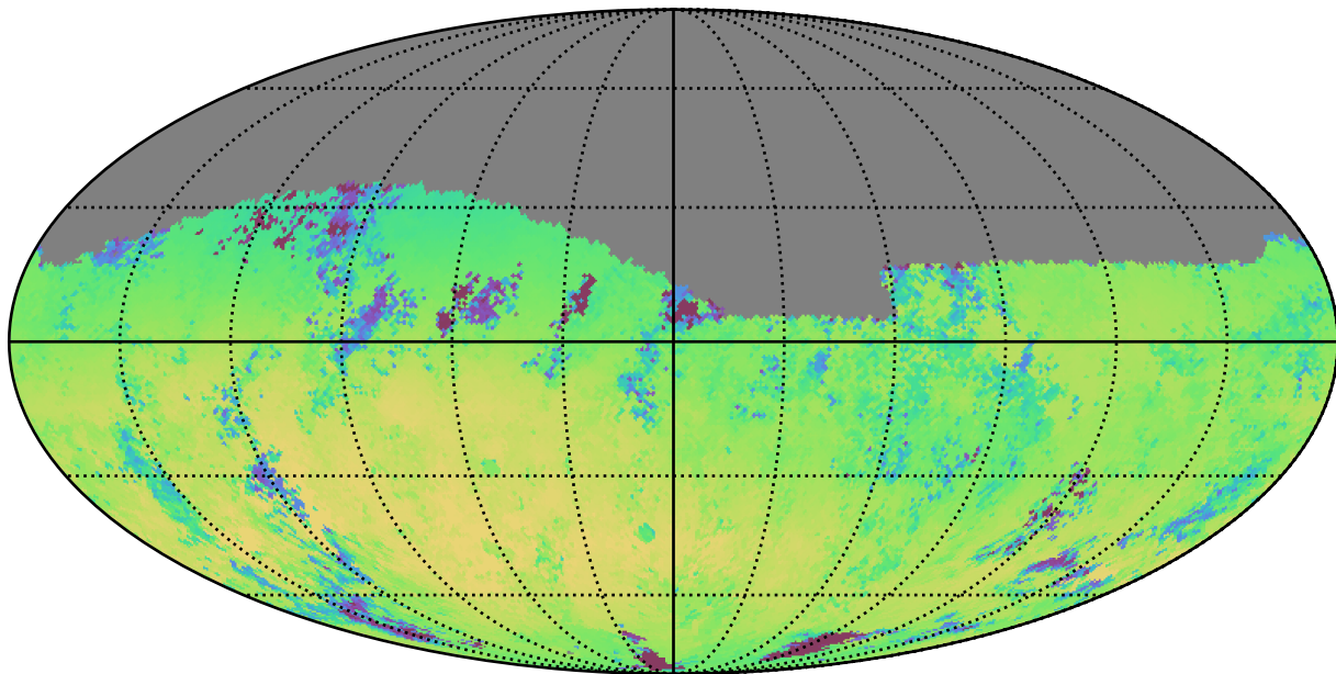
roll_pause_mjdp120_v3.4_10yrs Yr 1 r band: Median skyBrightness
