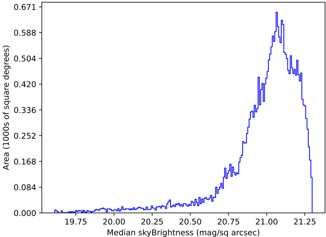
roll_pause_mjdp120_v3.4_10yrs Yr 1 r band: Median skyBrightness
