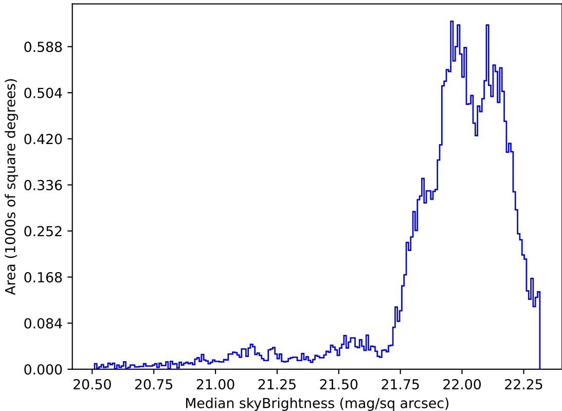
roll_pause_mjdp120_v3.4_10yrs Yr 1 g band: Median skyBrightness
