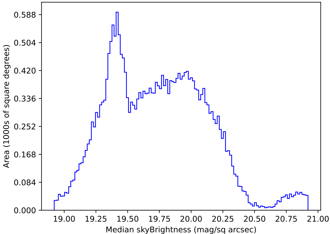
roll_pause_mjdp120_v3.4_10yrs Yr 1 all bands: Median skyBrightness
