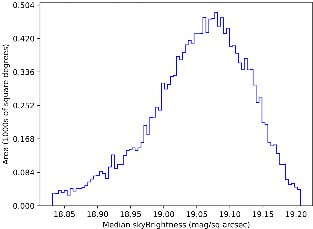
roll_pause_mjdp120_v3.4_10yrs WFD z band: Median skyBrightness
