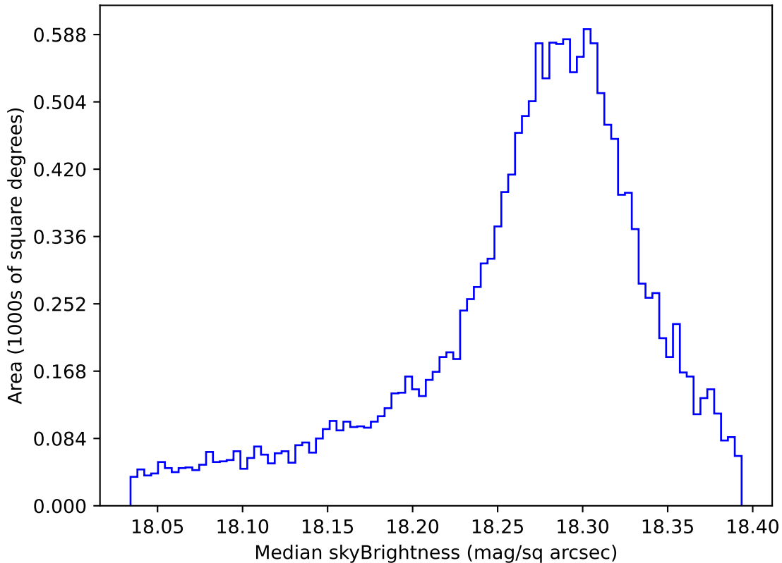
roll_pause_mjdp120_v3.4_10yrs WFD y band: Median skyBrightness
