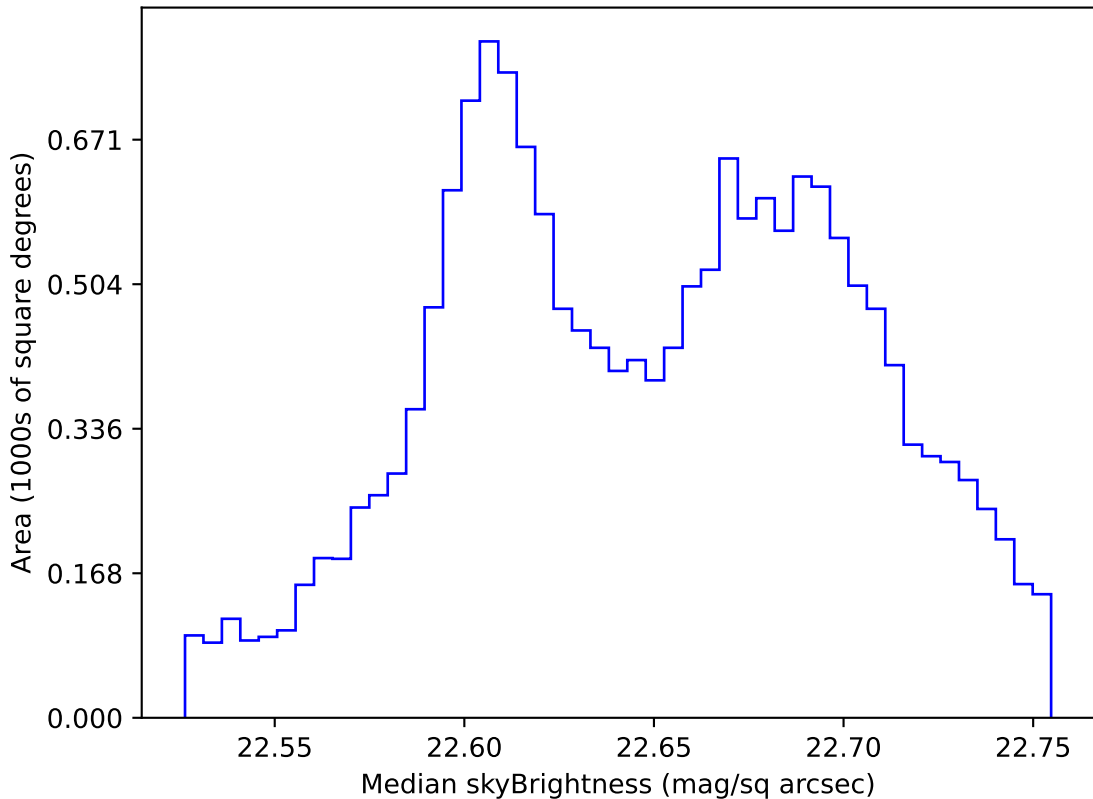
roll_pause_mjdp120_v3.4_10yrs WFD u band: Median skyBrightness
