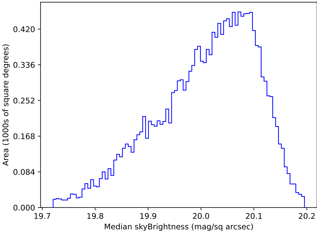
roll_pause_mjdp120_v3.4_10yrs WFD i band: Median skyBrightness
