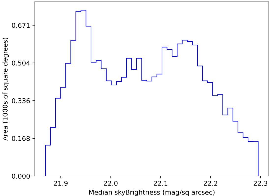
roll_pause_mjdp120_v3.4_10yrs WFD g band: Median skyBrightness
