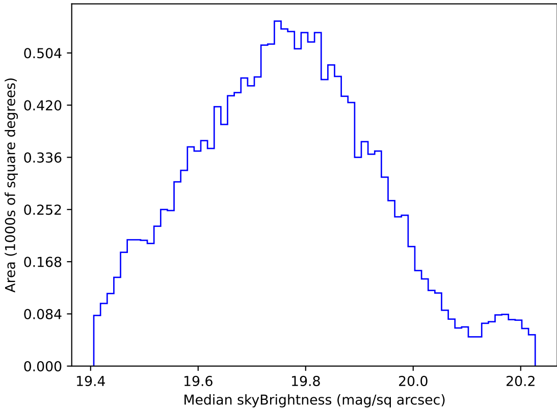
roll_pause_mjdp120_v3.4_10yrs WFD all bands: Median skyBrightness
