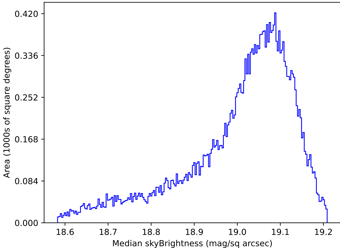
roll_pause_mjdp120_v3.4_10yrs All sky z band: Median skyBrightness
