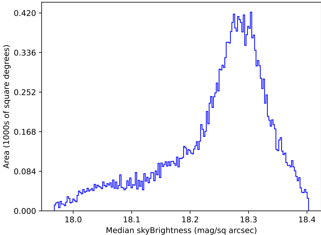
roll_pause_mjdp120_v3.4_10yrs All sky y band: Median skyBrightness
