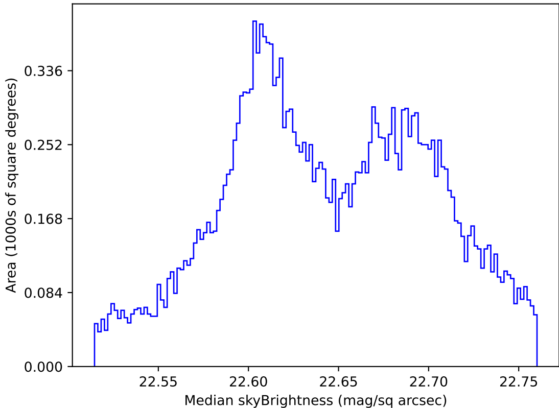
roll_pause_mjdp120_v3.4_10yrs All sky u band: Median skyBrightness
