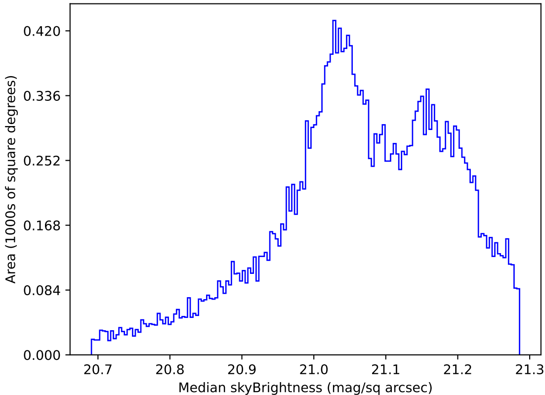
roll_pause_mjdp120_v3.4_10yrs All sky r band: Median skyBrightness
