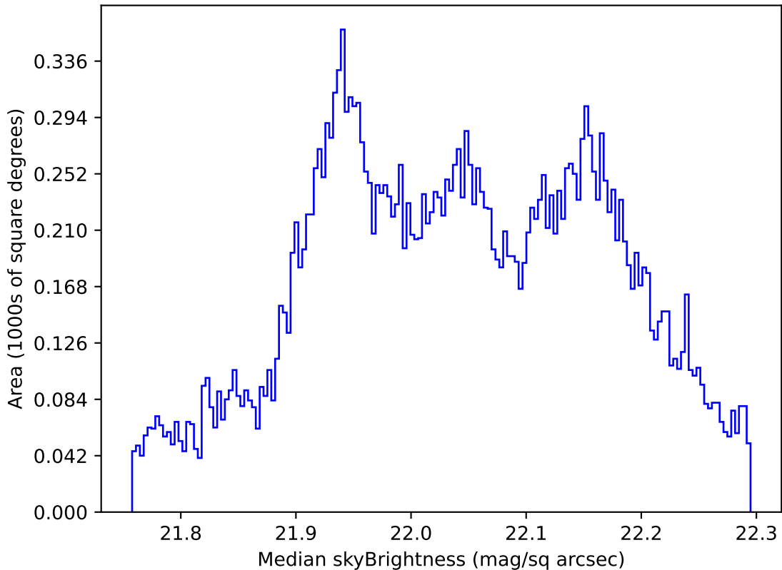
roll_pause_mjdp120_v3.4_10yrs All sky g band: Median skyBrightness
