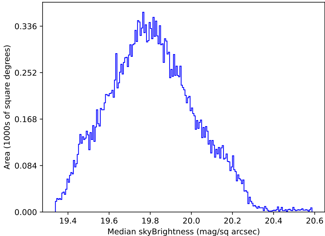
roll_pause_mjdp120_v3.4_10yrs All sky all bands: Median skyBrightness
