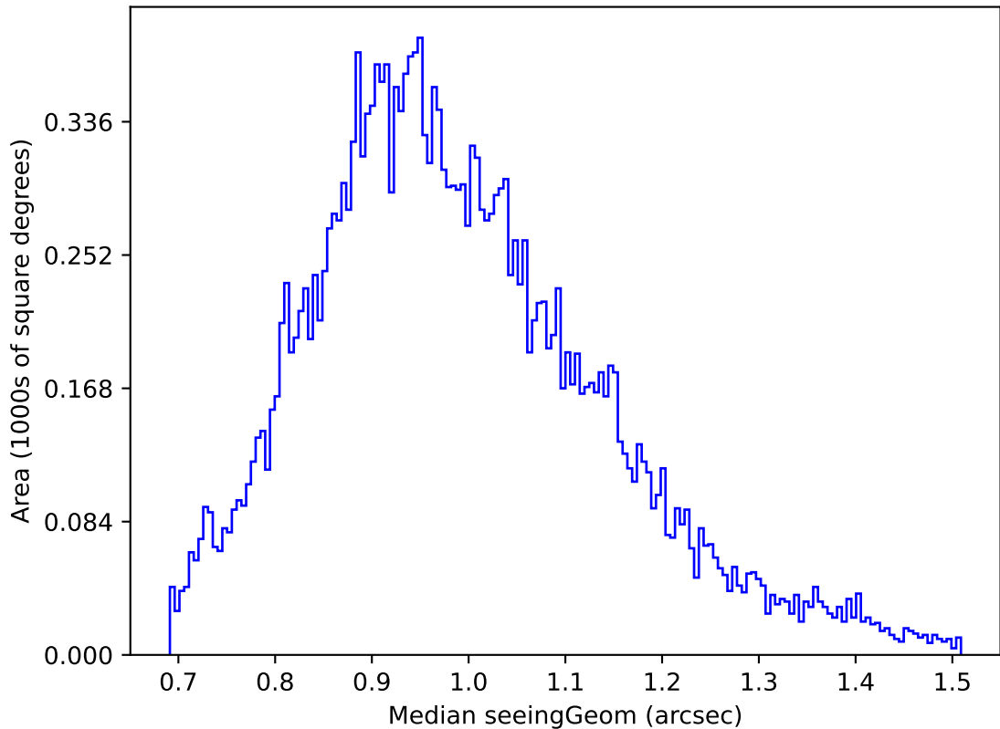
roll_pause_mjdp120_v3.4_10yrs Yr 1 u band: Median seeingGeom
