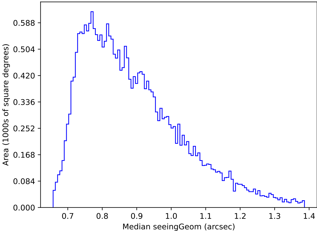
roll_pause_mjdp120_v3.4_10yrs Yr 1 r band: Median seeingGeom
