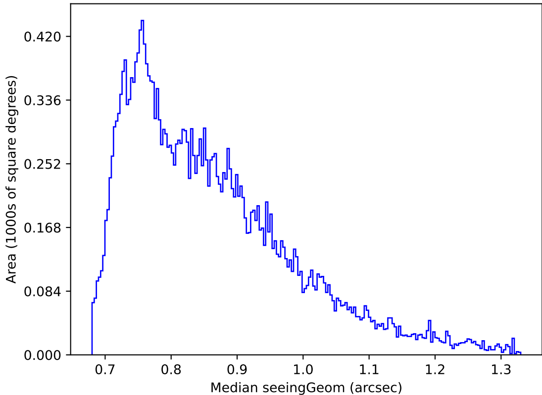
roll_pause_mjdp120_v3.4_10yrs Yr 1 i band: Median seeingGeom
