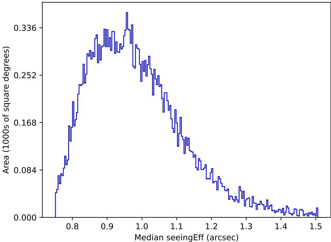
roll_pause_mjdp120_v3.4_10yrs Yr 1 z band: Median seeingEff
