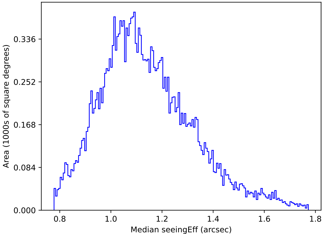
roll_pause_mjdp120_v3.4_10yrs Yr 1 u band: Median seeingEff
