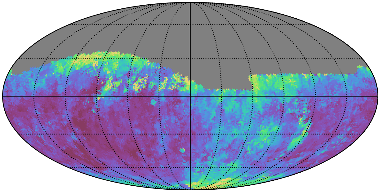
roll_pause_mjdp120_v3.4_10yrs Yr 1 r band: Median seeingEff
