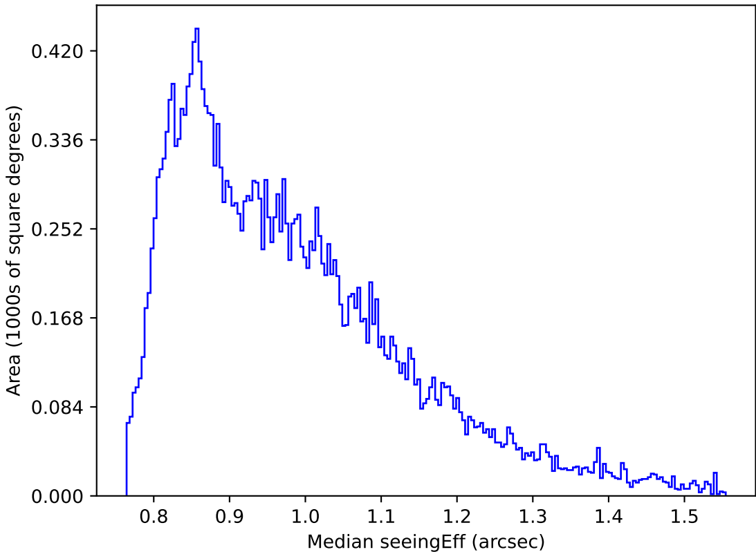
roll_pause_mjdp120_v3.4_10yrs Yr 1 i band: Median seeingEff
