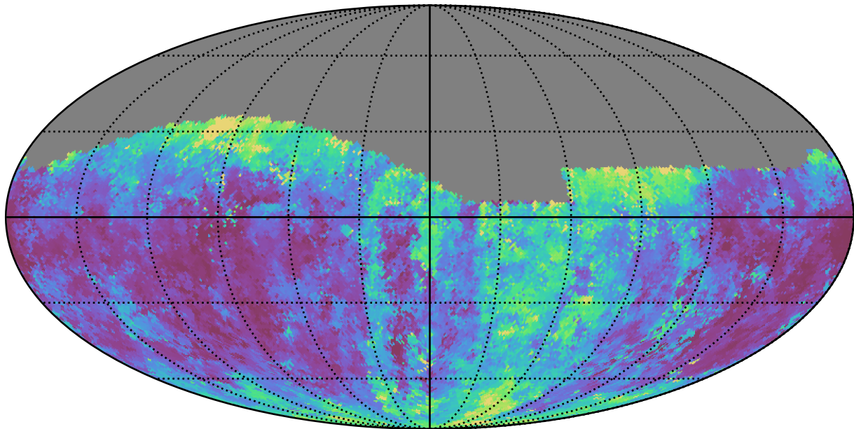
roll_pause_mjdp120_v3.4_10yrs Yr 1 g band: Median seeingEff
