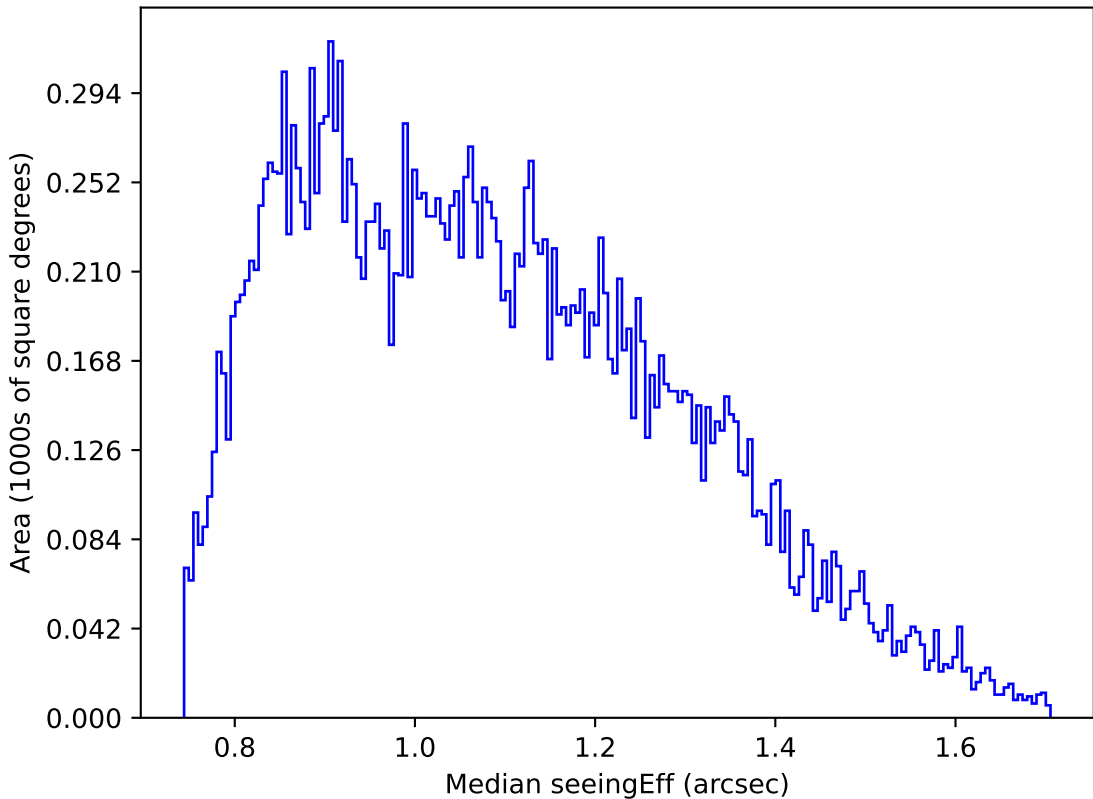
roll_pause_mjdp120_v3.4_10yrs Yr 1 g band: Median seeingEff
