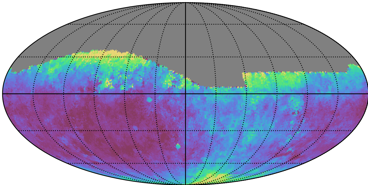
roll_pause_mjdp120_v3.4_10yrs Yr 1 all bands: Median seeingEff
