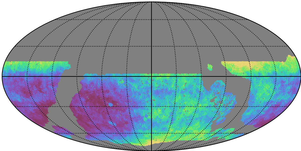
roll_pause_mjdp120_v3.4_10yrs WFD z band: Median seeingEff
