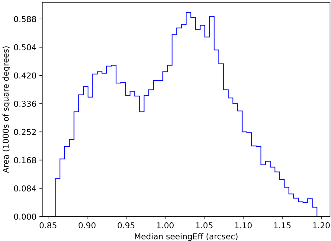
roll_pause_mjdp120_v3.4_10yrs WFD z band: Median seeingEff
