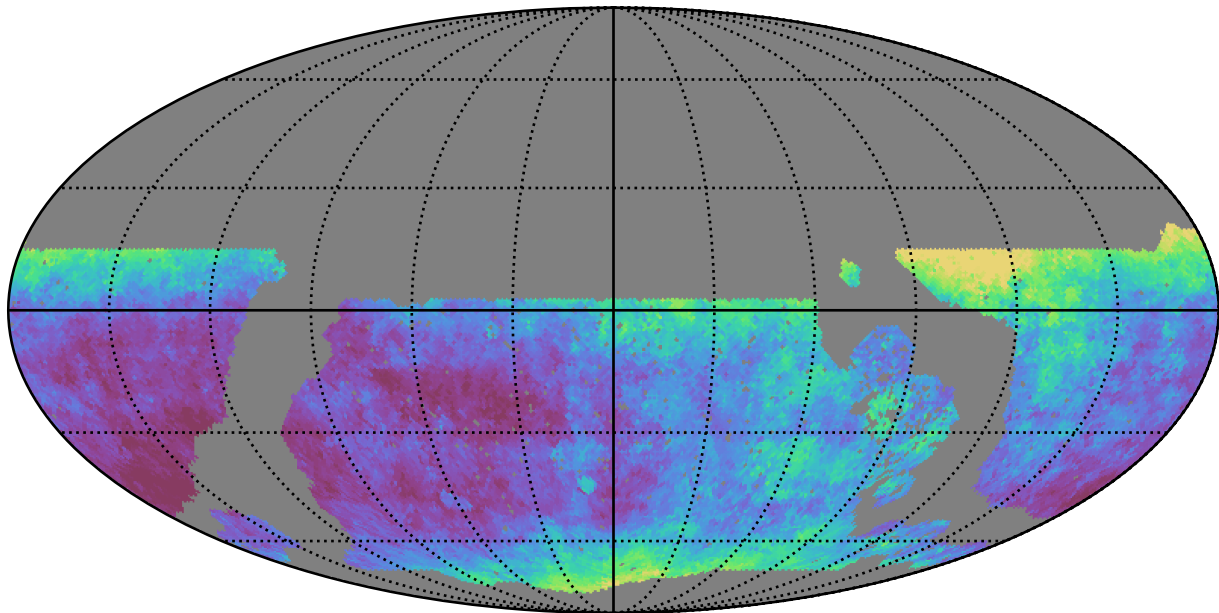
roll_pause_mjdp120_v3.4_10yrs WFD y band: Median seeingEff
