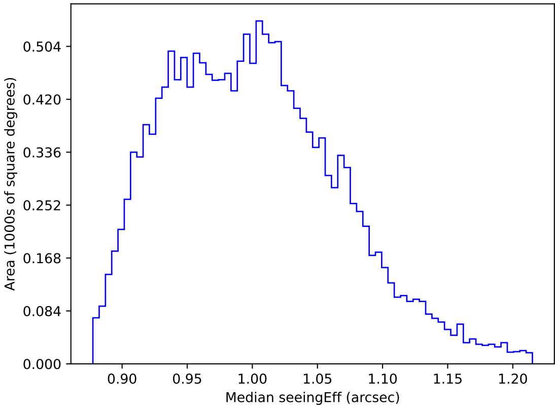
roll_pause_mjdp120_v3.4_10yrs WFD y band: Median seeingEff
