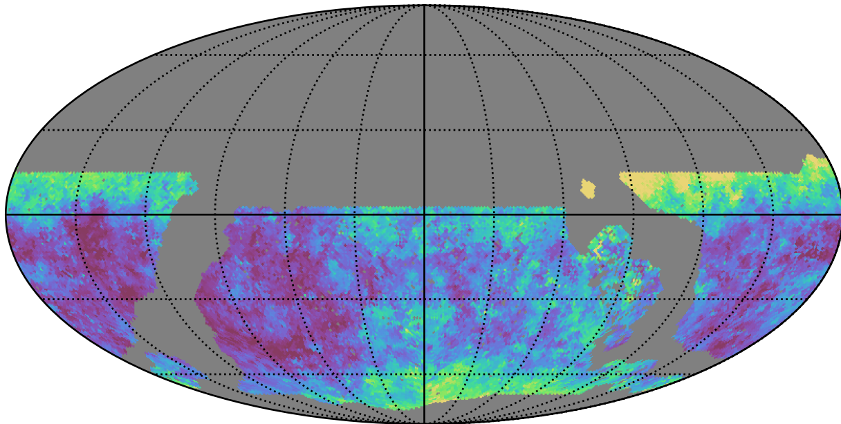
roll_pause_mjdp120_v3.4_10yrs WFD u band: Median seeingEff
