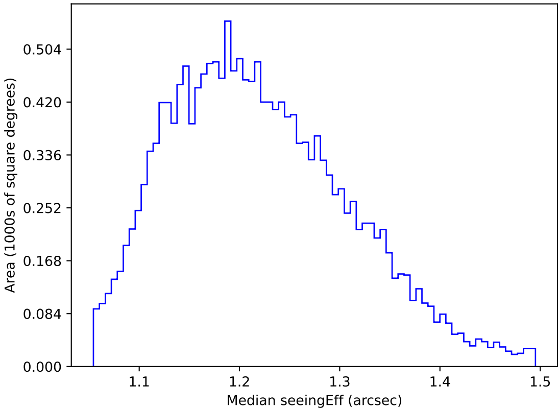
roll_pause_mjdp120_v3.4_10yrs WFD u band: Median seeingEff
