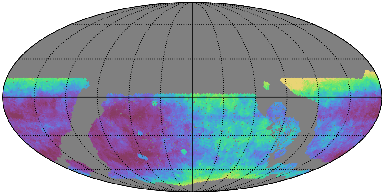
roll_pause_mjdp120_v3.4_10yrs WFD r band: Median seeingEff
