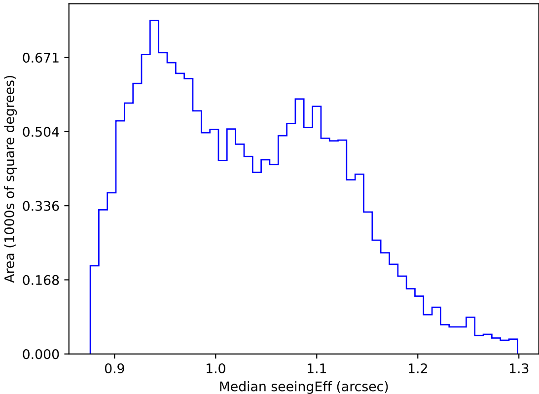
roll_pause_mjdp120_v3.4_10yrs WFD r band: Median seeingEff
