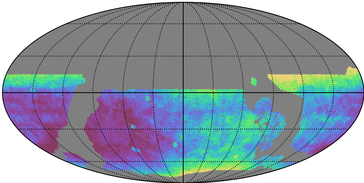
roll_pause_mjdp120_v3.4_10yrs WFD i band: Median seeingEff
