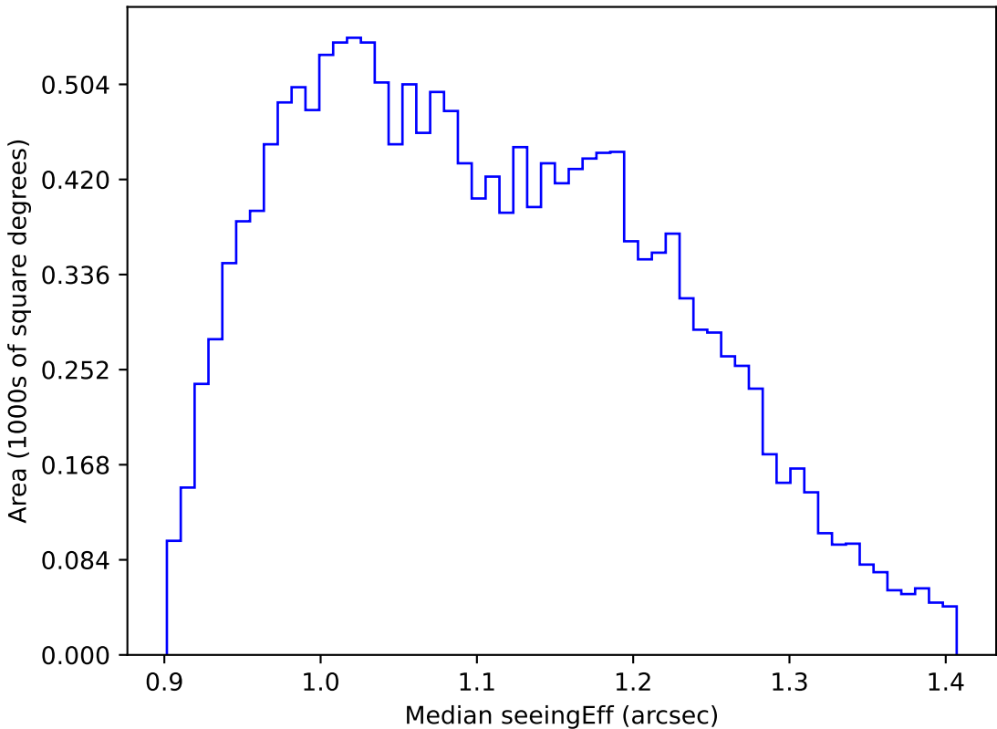
roll_pause_mjdp120_v3.4_10yrs WFD g band: Median seeingEff
