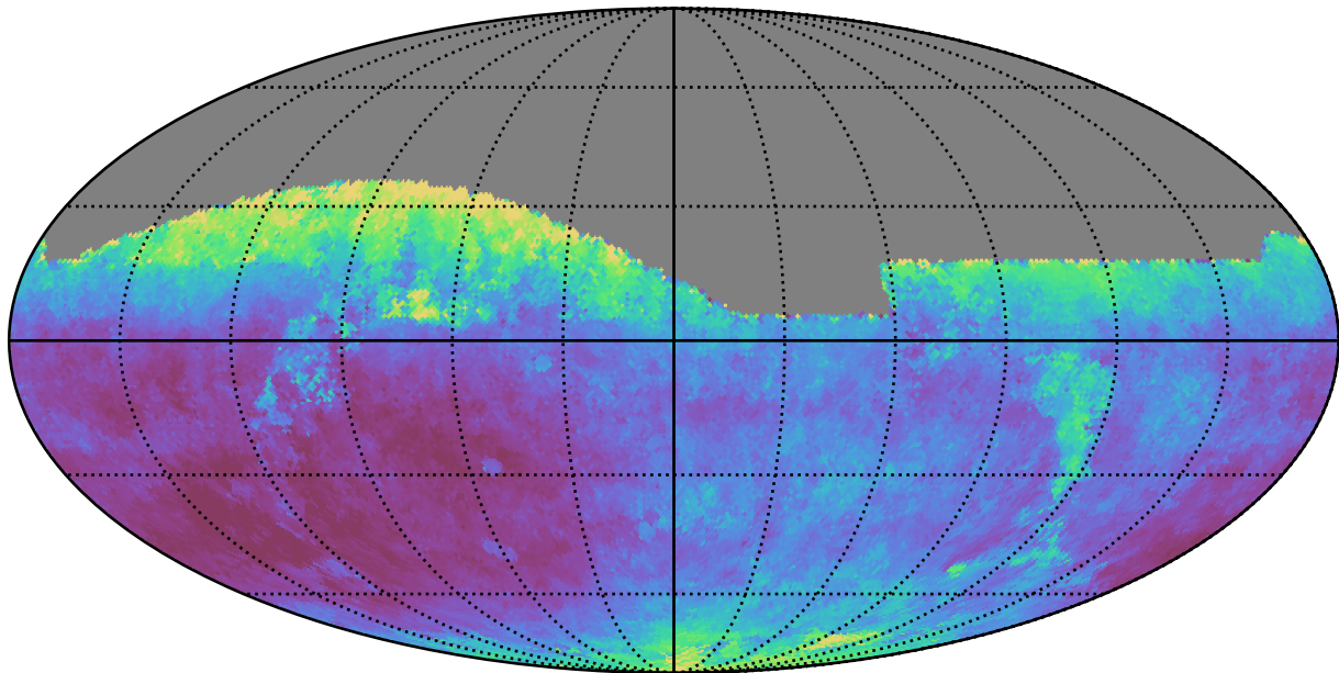
roll_pause_mjdp120_v3.4_10yrs All sky z band: Median seeingEff
