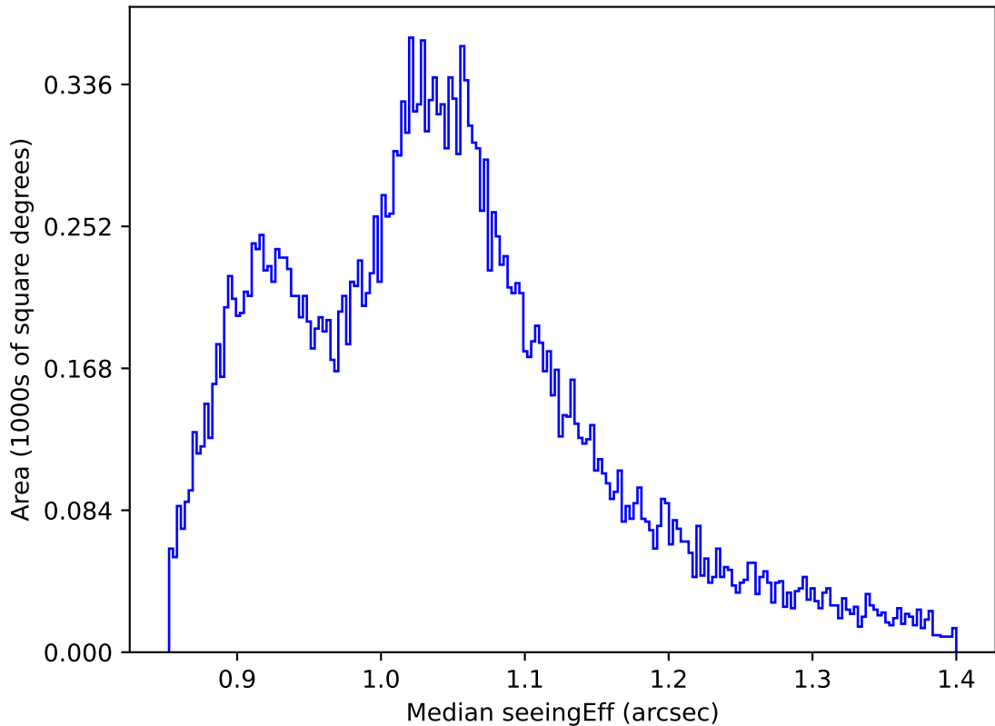
roll_pause_mjdp120_v3.4_10yrs All sky z band: Median seeingEff
