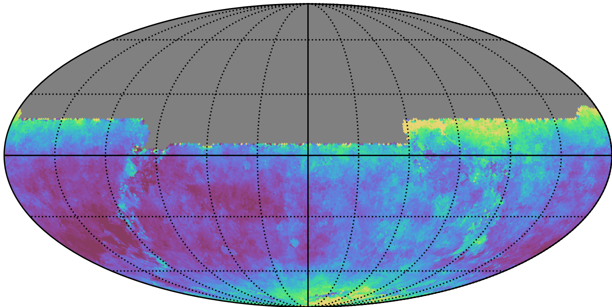
roll_pause_mjdp120_v3.4_10yrs All sky y band: Median seeingEff
